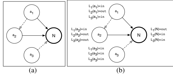
Fig. 2. Flatmates example: (a) TODF's associated graph; (b) TODF together with labellings.
