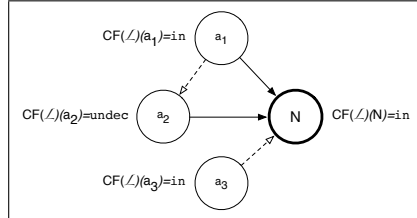
Fig. 3. Flatmates example: aggregated labellings (and decision over target N ) computed by CF .
